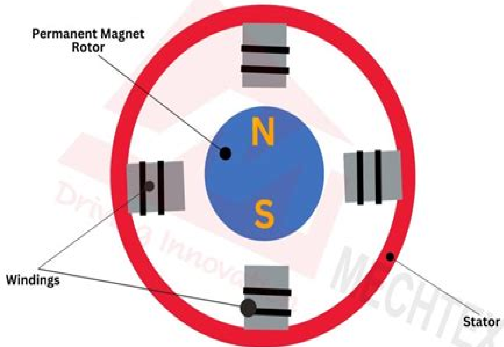
Synchronous Motor
