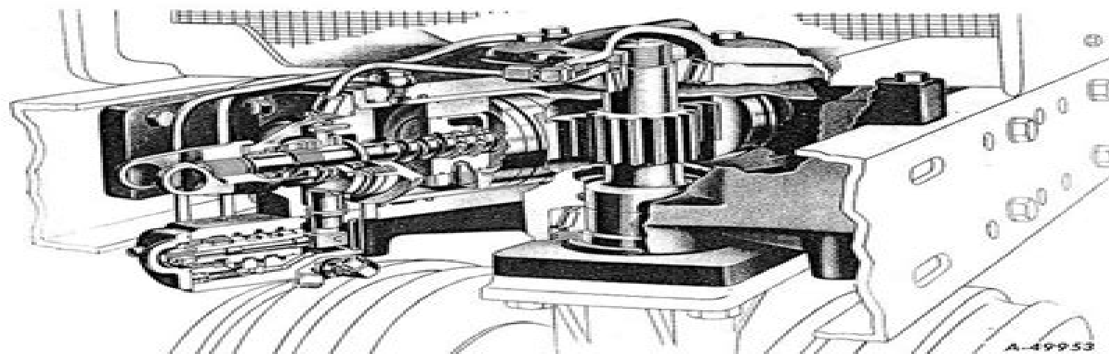
Blas. 9. Cut-away view of the steering mechanism of a Ford 460 tractor.
