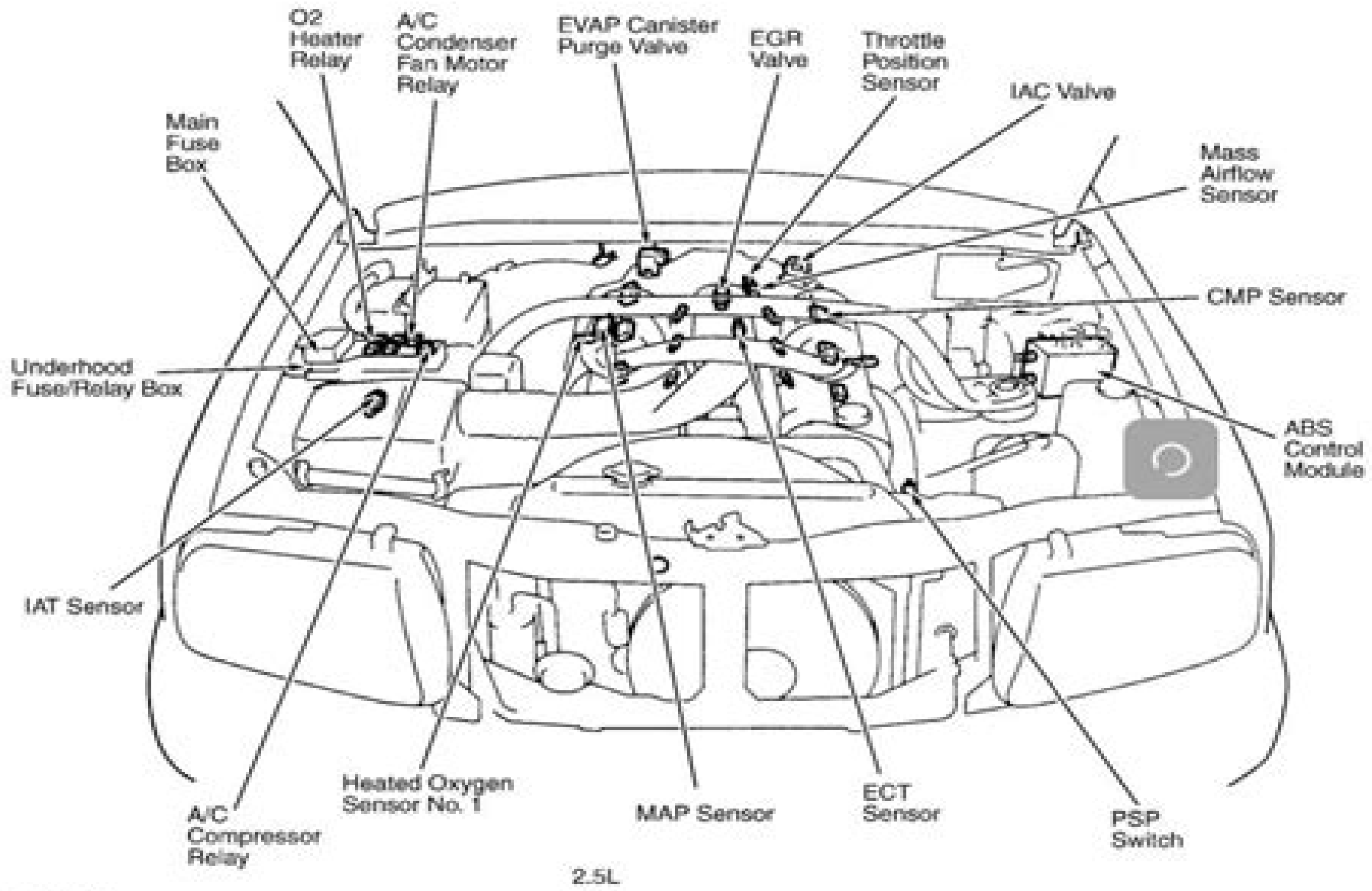
Fig. 1: Engine Compartment (2.5L)
