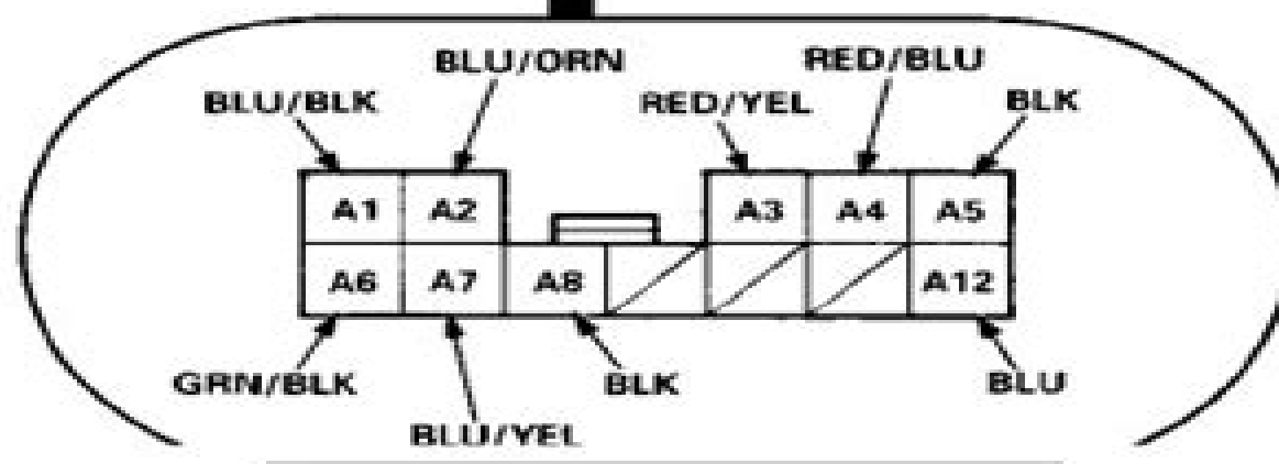
Wire side of female terminals
