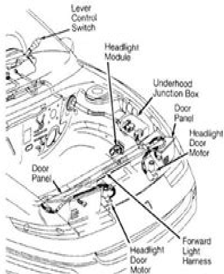
Fig. 4: Headlight Door Component Locations (SC1 & SC2)
