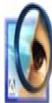
Version 7
