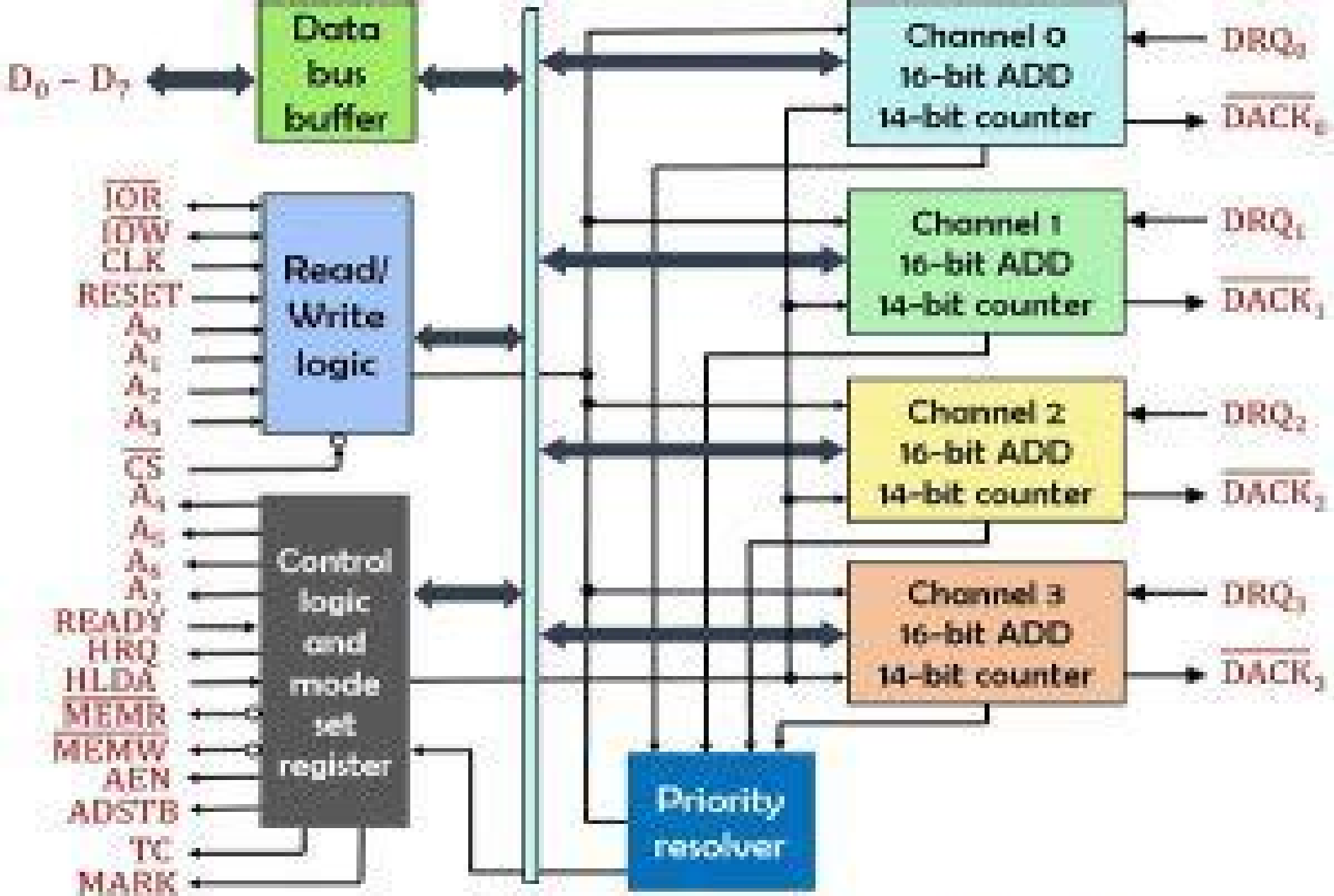
Architecture of 8257 DMA Controller
