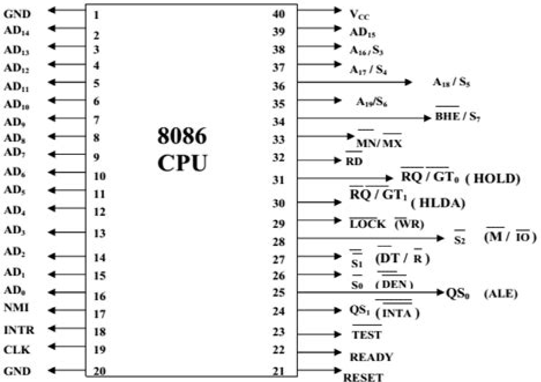
Pin Diagram of 8086
