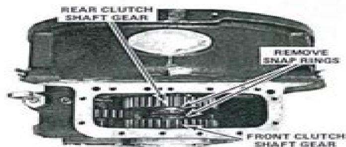
FIGURE 50 - Top View of Transmission
