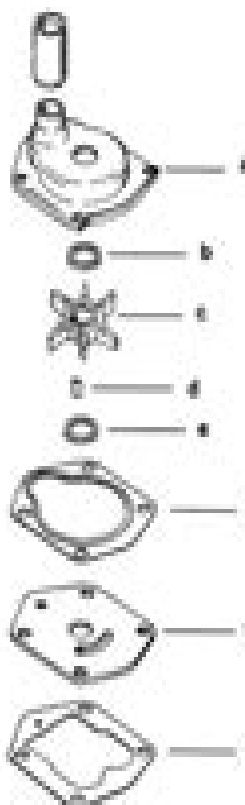
a - Cover b - Washer (above impeller) c - Impeller d - Key e - Washer (below impeller) f - Cover Gasket g - Base Plate h - Base Gasket
