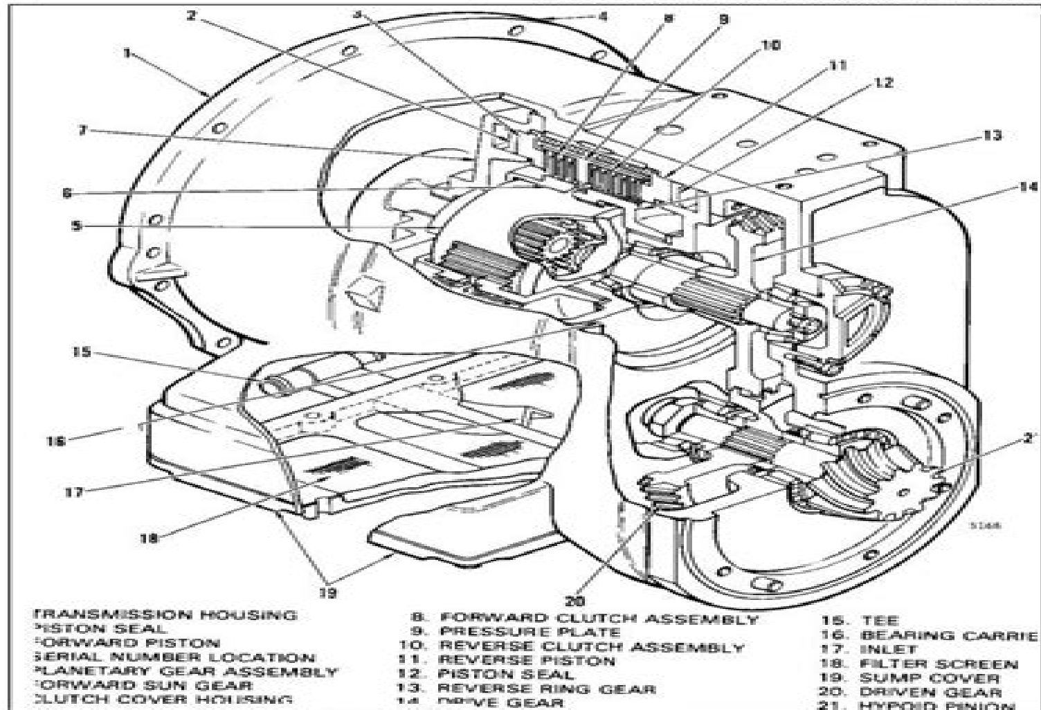
FIGURE 1. POWERSHIFT TRANSMISSION
