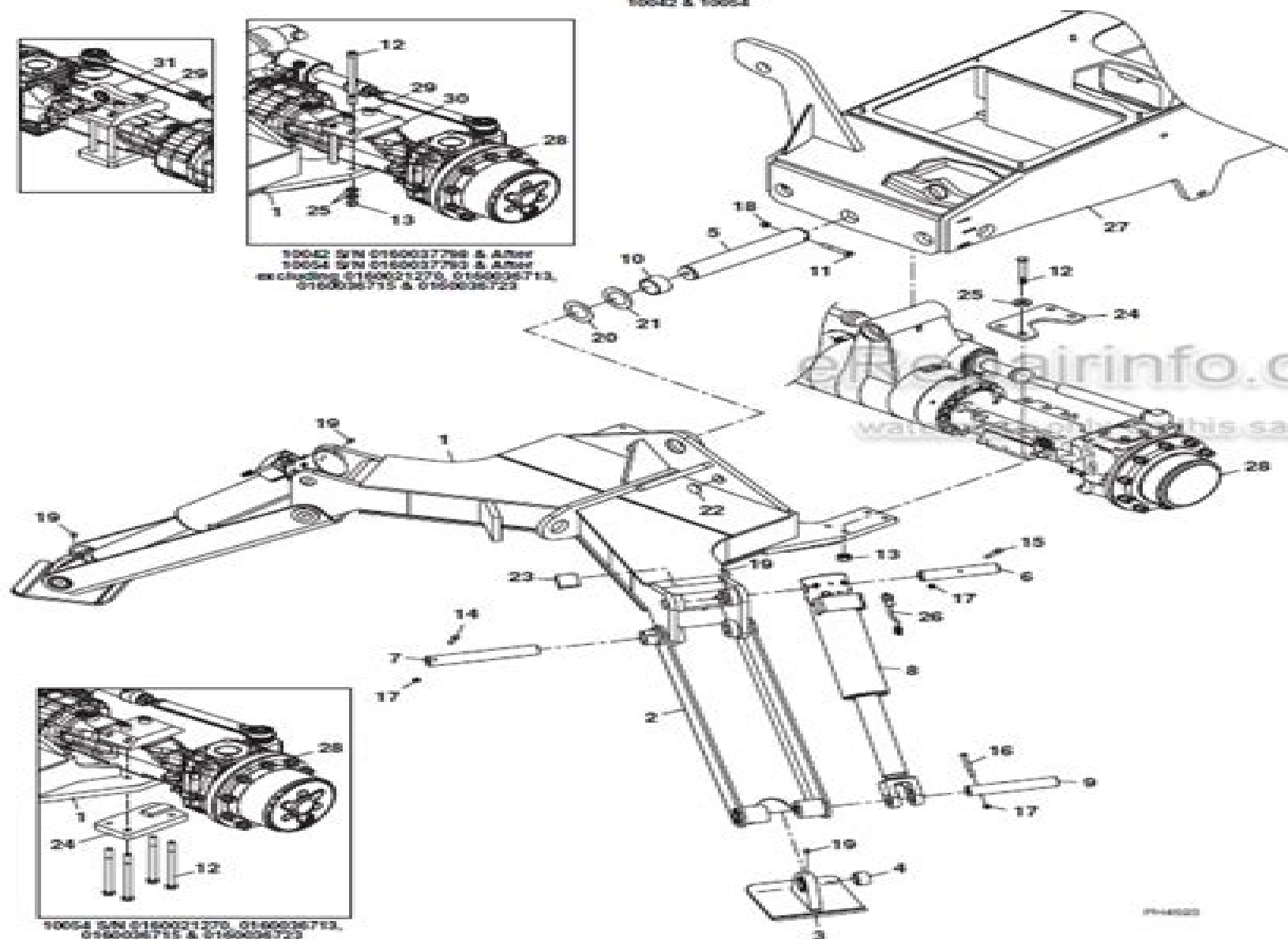
Figure 1-3 Outrigger Mounting
