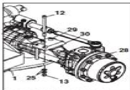
Figure 1-3 Outrigger Mounting
