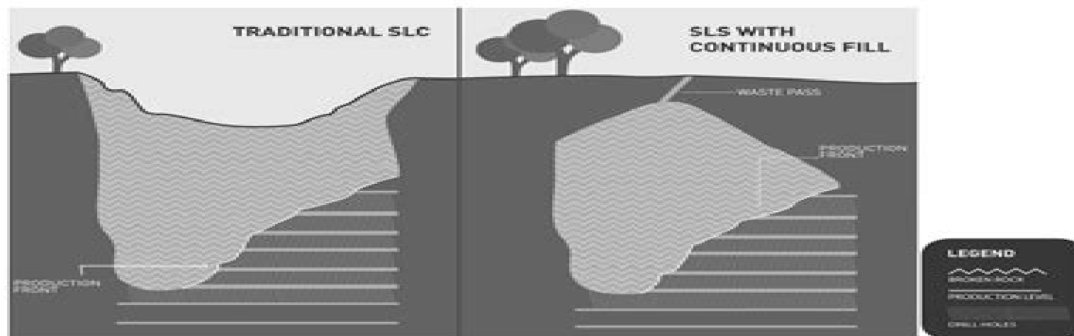
FIG 1 – Sublevel cave (showing caving of the overlying strata) versus sublevel shrinkage with continuous fill (caving of the overlying strata is minimised).
