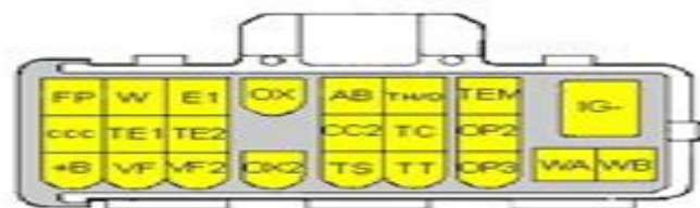
23 pin Toyota diagnostic connector
