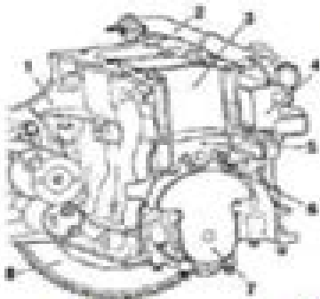
Fig. 1.19. Cooling of the piston: 1 - the engine block, 2 - pipe cooling system, 3 - cylinder walls, 4 - oil cooler, 5 - piston, 6 - oil spray atomizer, 7 - crankshaft
