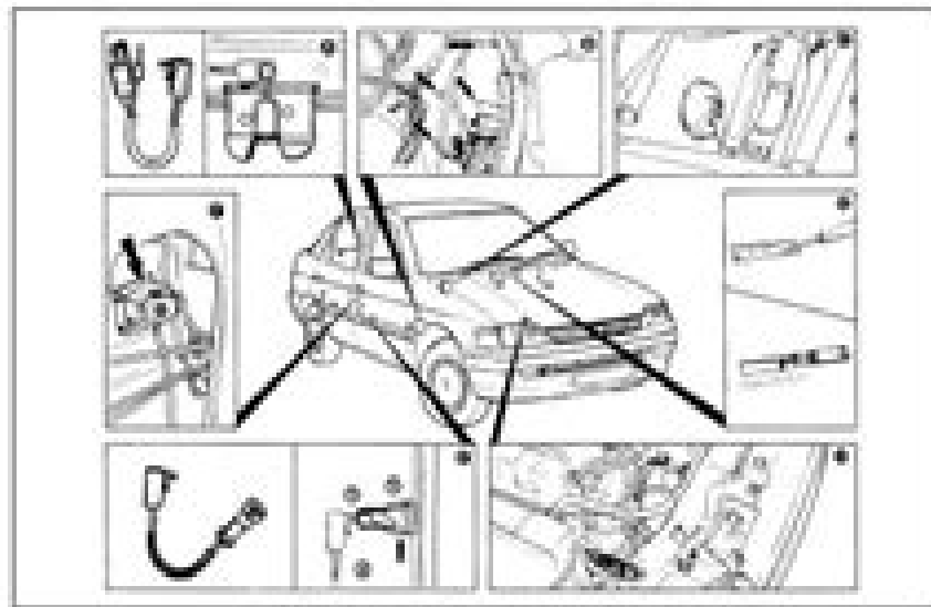
21.1 Anti-theft alarm system components and their locations
