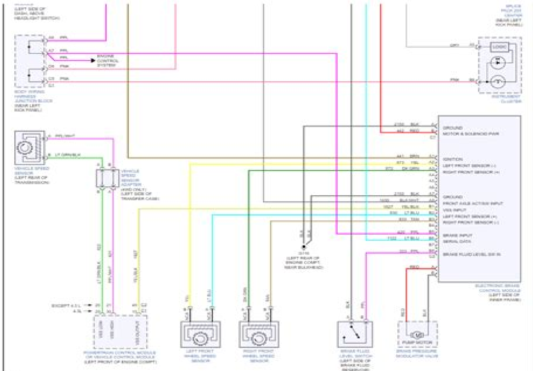
Fig 1: Anti-lock Brakes Circuit
