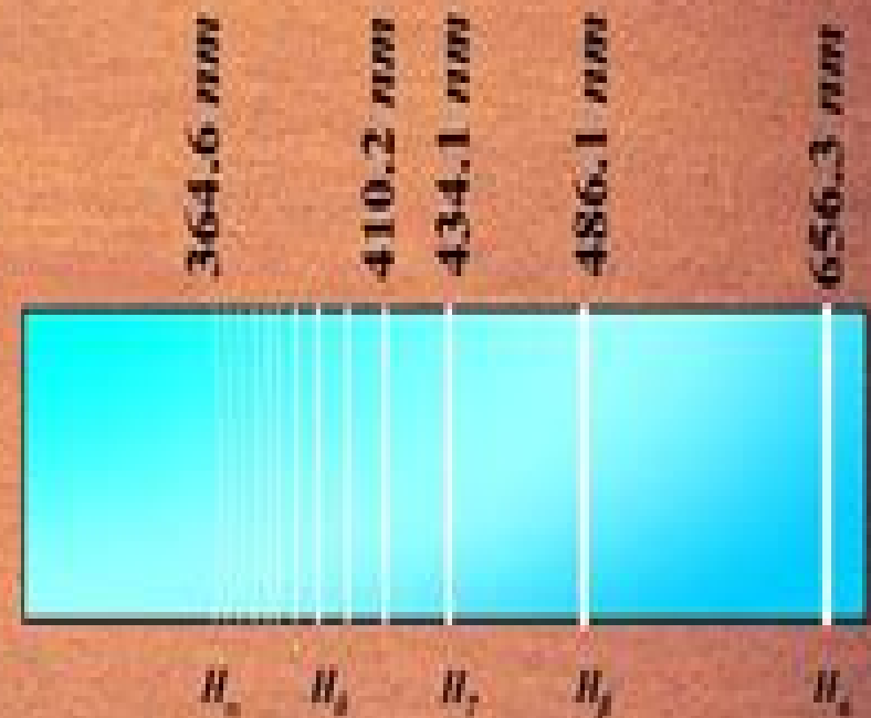
Balmer series in the emission spectrum of hydrogen
