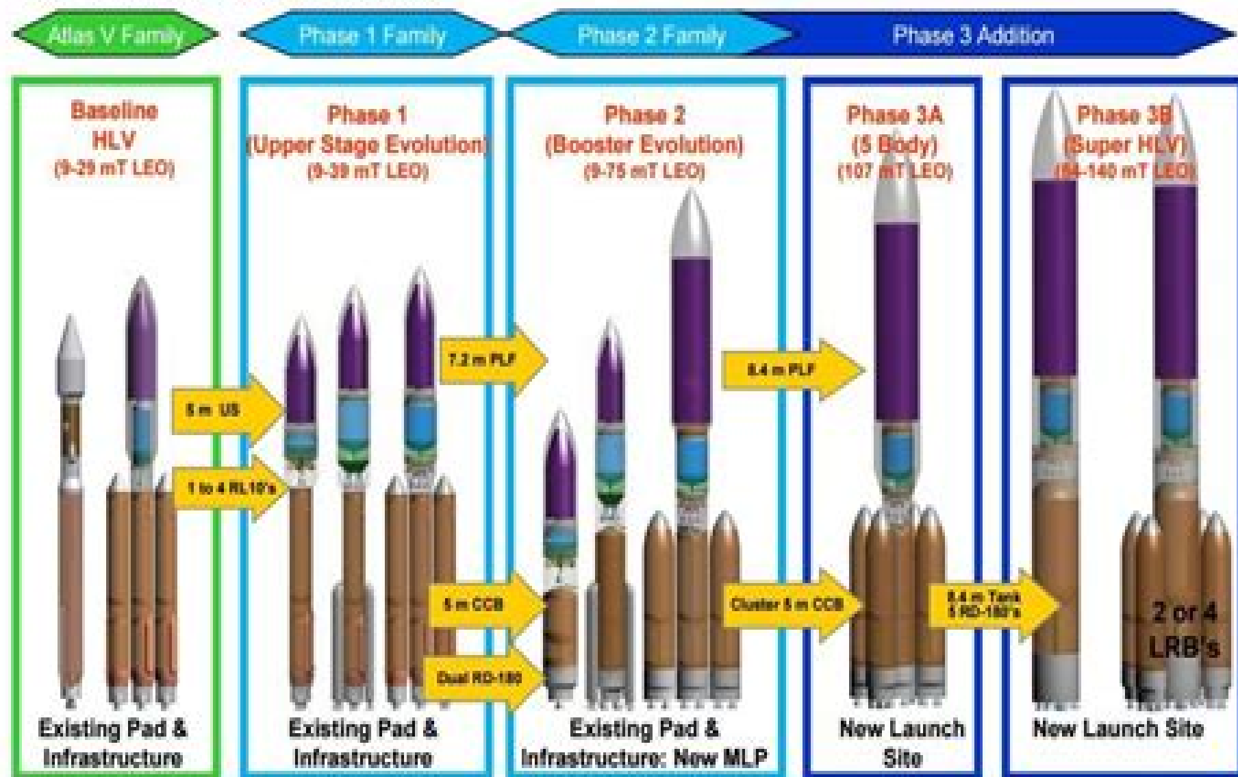
Figure 8.2.3-1: Heavy-Lift Evolution
