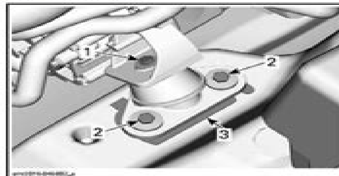
REAR STARBOARD ENGINE MOUNT SHOWN 1. Engine mounting screw 2. Engine mount retaining screw 3. Shim(s)
