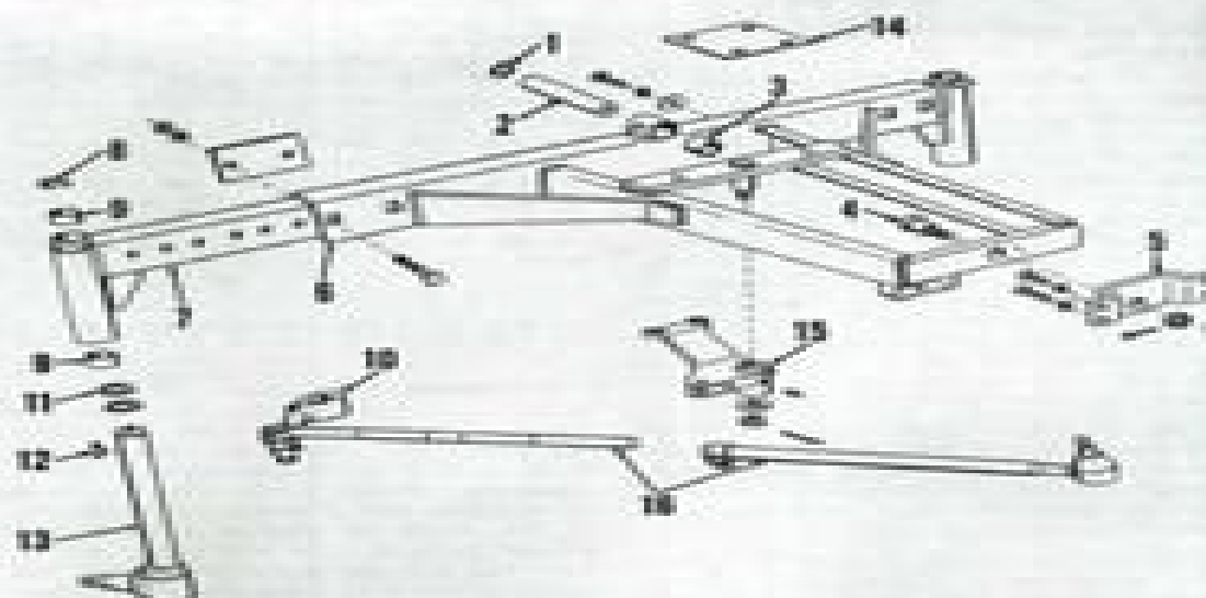
Fig. 5—Exploded view of adjustable front axle assembly used on all models except 7000. Steering arm (14) is used with internal cylinder type front support (Fig. 12). Steering arm (15) is used with external cylinder type steering (Fig. 13).
