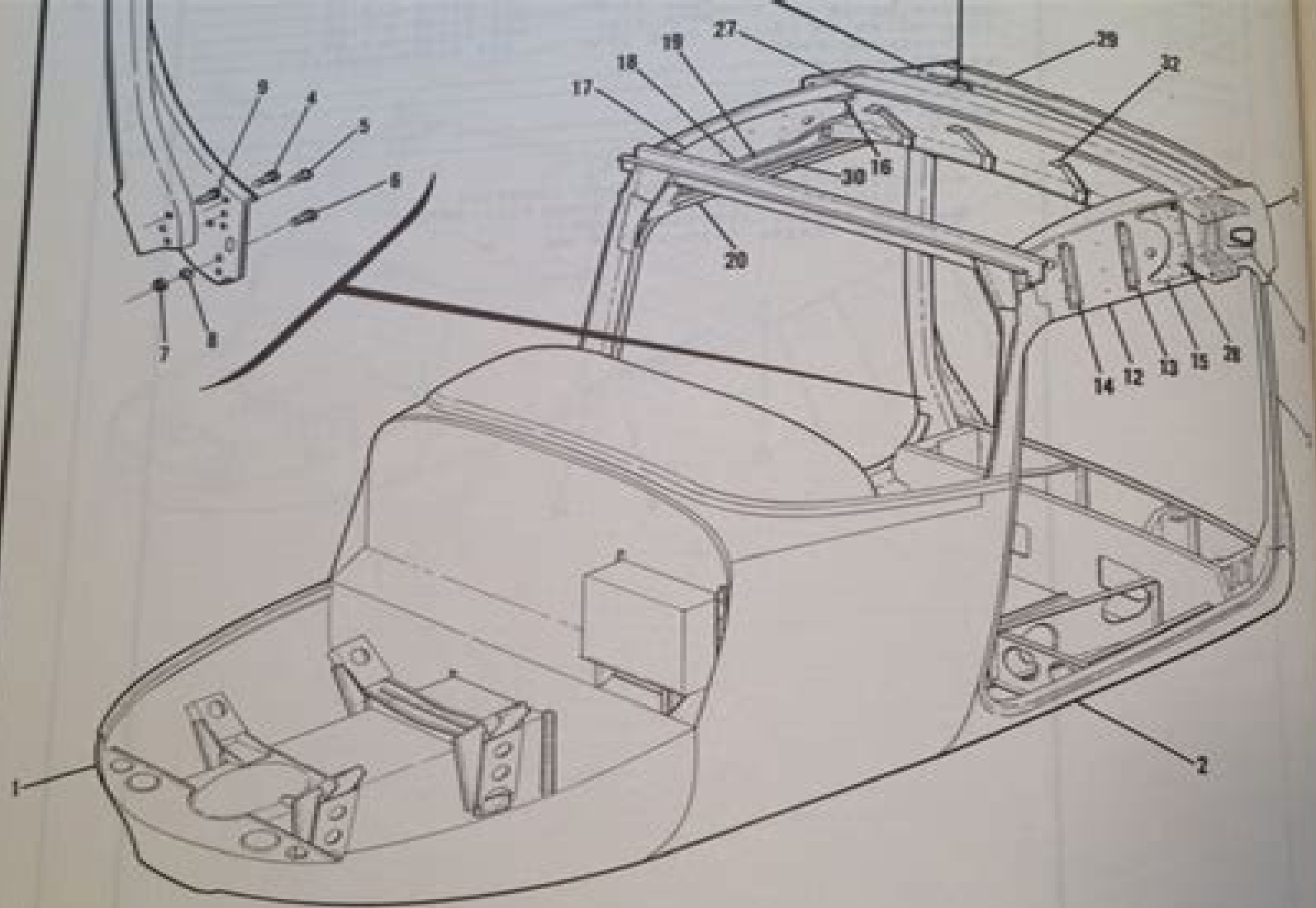
Figure 14. Front & Center Section Assembly
