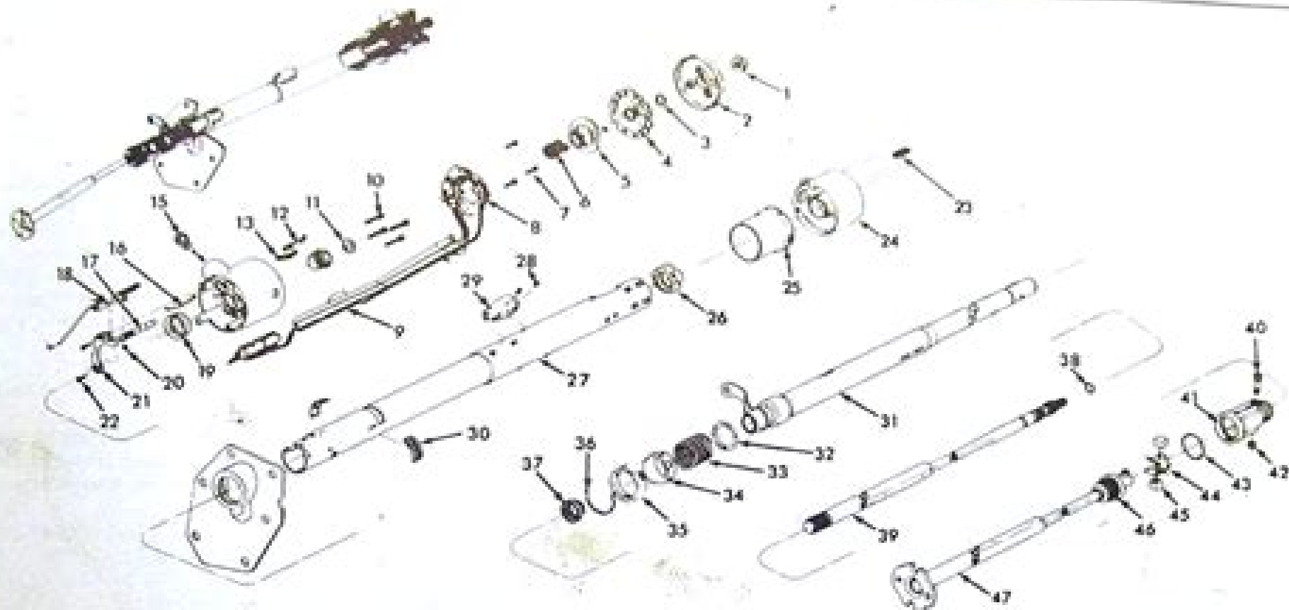
Fig. 11.19 Standard steering column components (Sec 26)
