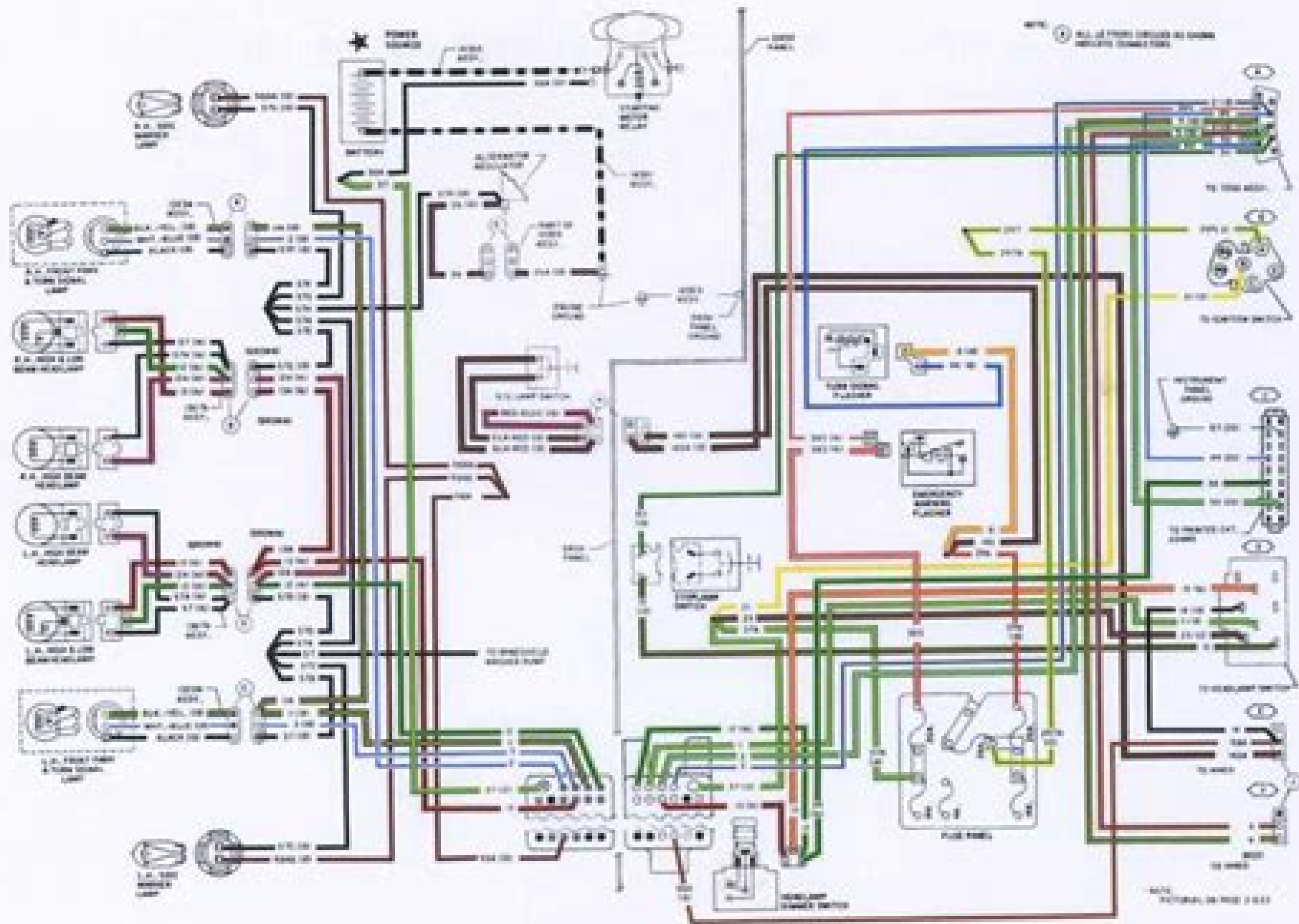
1969 MUSTANG EXTERIOR LIGHTS,TURN SIGNALS AND BRAKE LIGHTS
