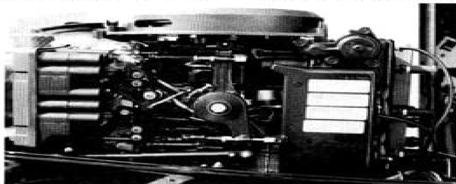
Front of a 1967 60hp greenhead. A practical maintenance and tuning program followed throughout the year, is one of the best methods of ensuring the engine will give satisfactory performance at any time.
