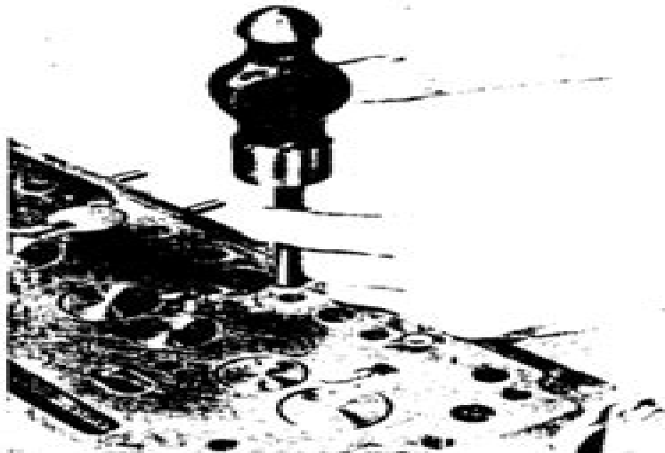
Fig. 13 - Securing the Welch Plug in Place
