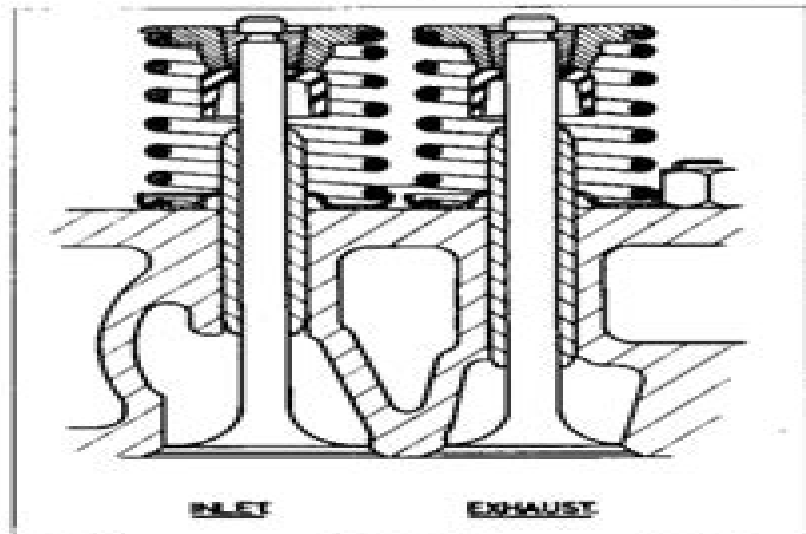
Fig. 14 - Cross Sectional View of Intake and Exhaust Valve Arrangement
