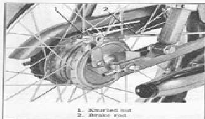
Figure 30-41. Rear Brake Adjustment, M, MS, MC, X, Z
