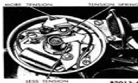
FIG. 24—Adjusting Breaker Point Spring Tension
