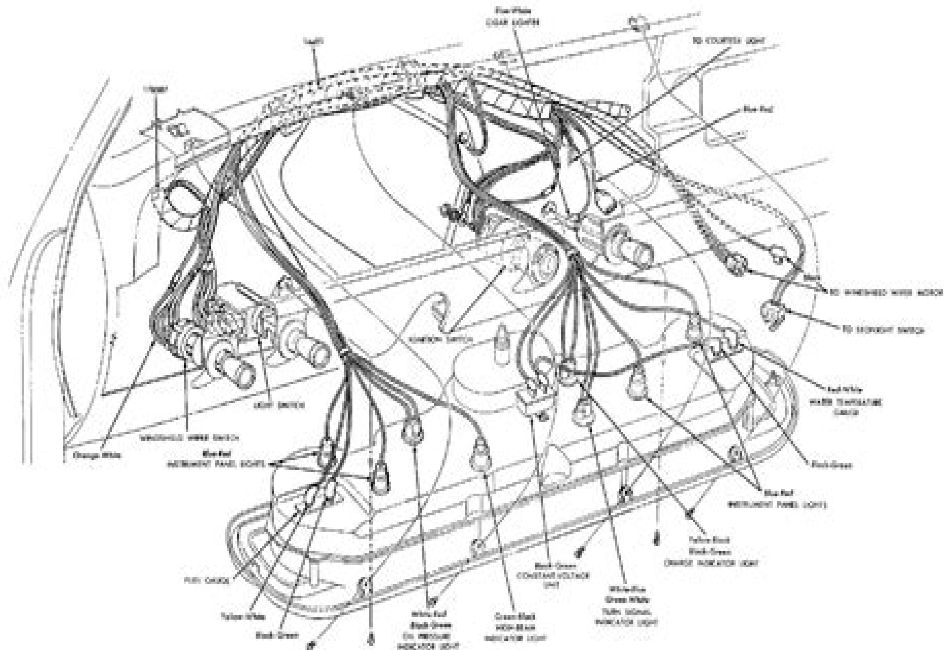
1965 MUSTANG INSTRUMENT PANEL WITH ALTERNATOR CHARGING SYSTEM
