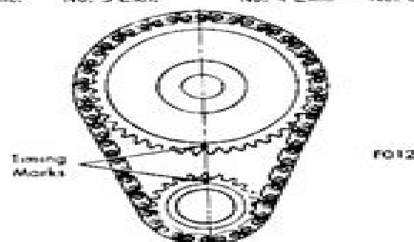
170", 200", 250" VALVE TIMING MARKS
