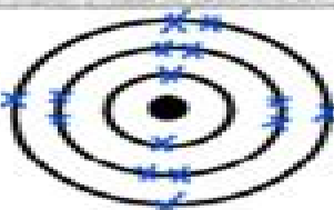
Phosphorus atom
