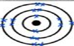
Chlorine atom
