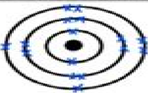
Sulfur atom
