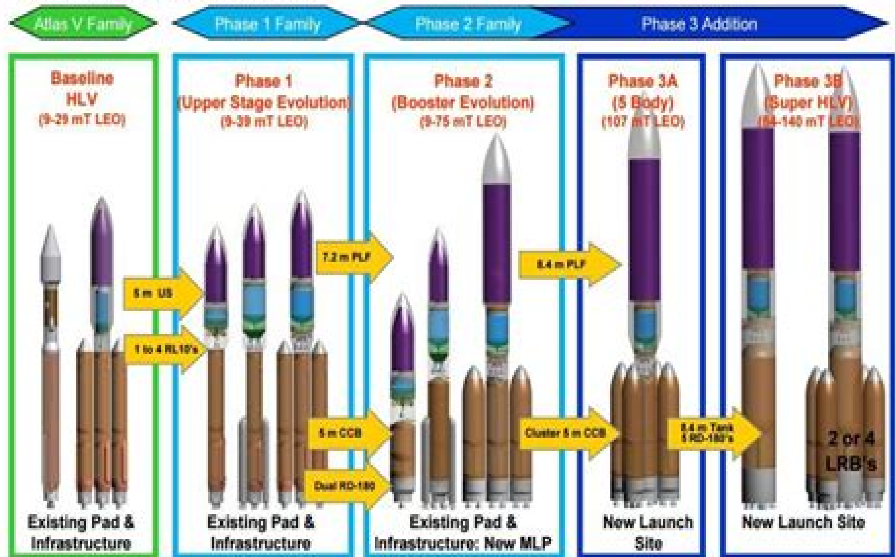
Figure 8.2.3-1: Heavy-Lift Evolution
