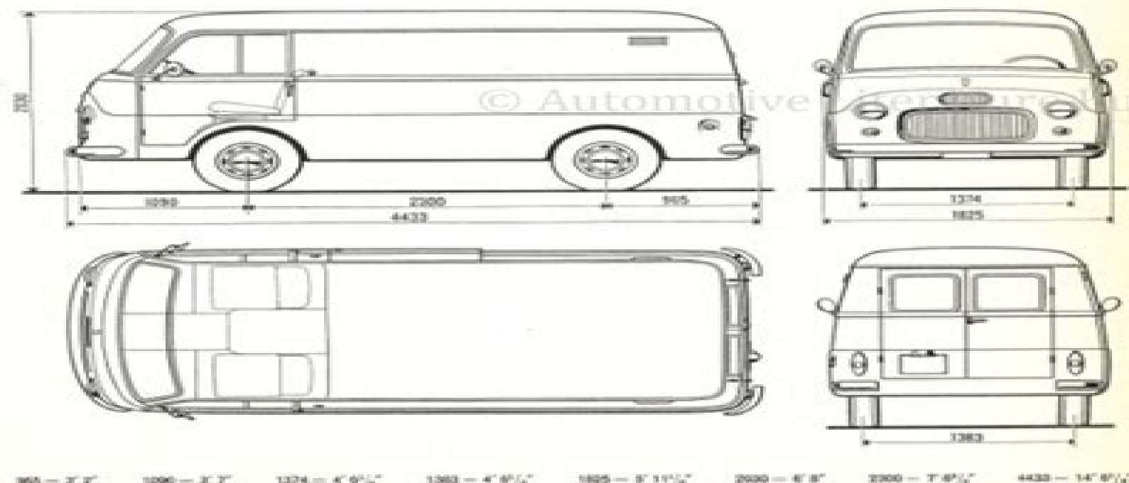
Fig. 2. - Main dimensions of the Van model 1100 T (type 217 D).
