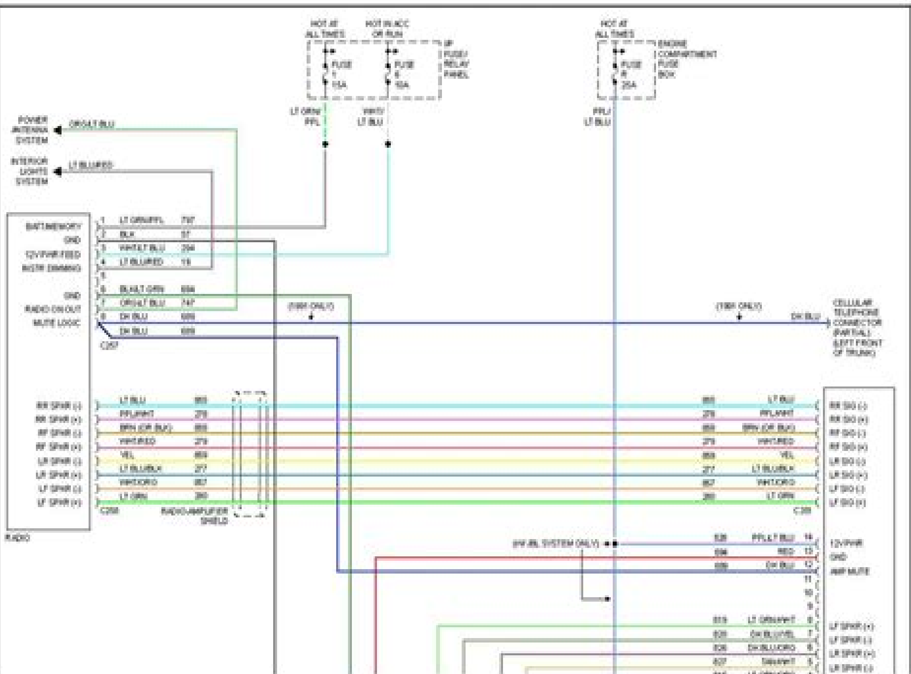
1990 Lincoln Town Car-Fig. 13: Radio Circuits
