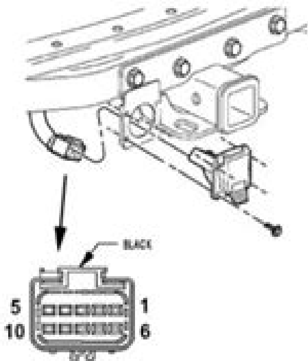
Rear hitch 10-pin connector
