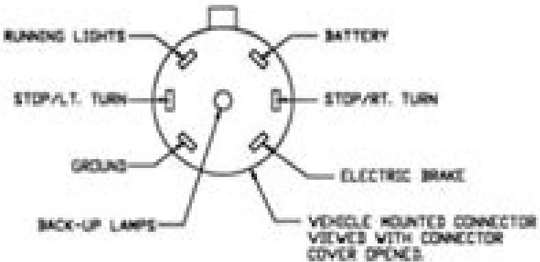
Rear connector #1 (7 way)
