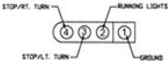
Rear connector #2 (4 way)
