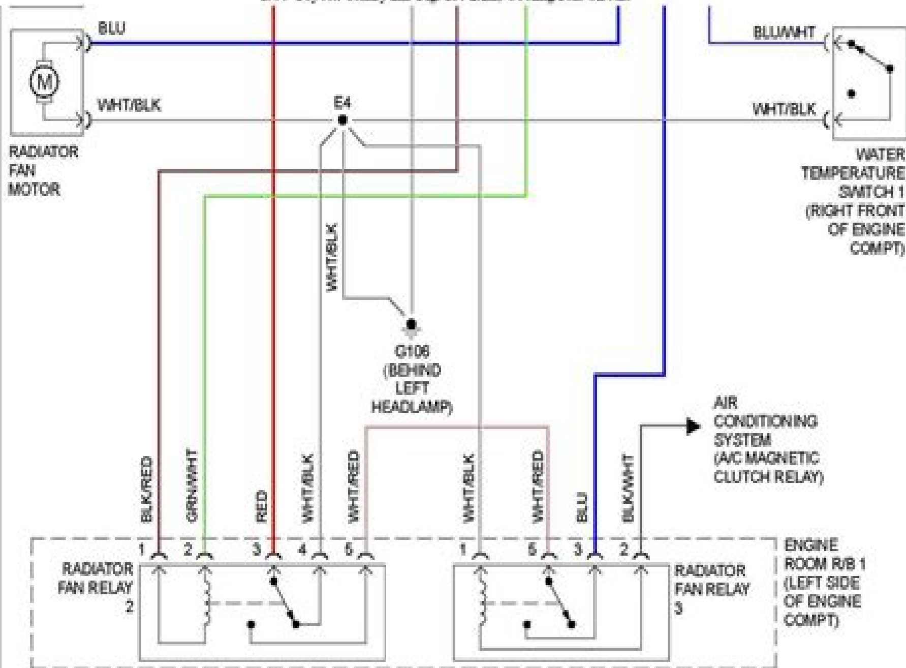
1999 Toyota Camry LE-Fig. 15: 2.2L, Cooling Fan Circuit
