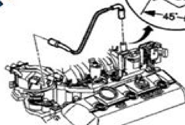
Fig. J70: Ignition Coil Wire Courtesy of GENERAL MOTORS CORP.
