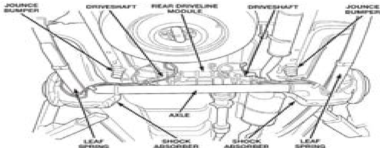
Fig. 2 All Wheel Drive Rear Suspension
