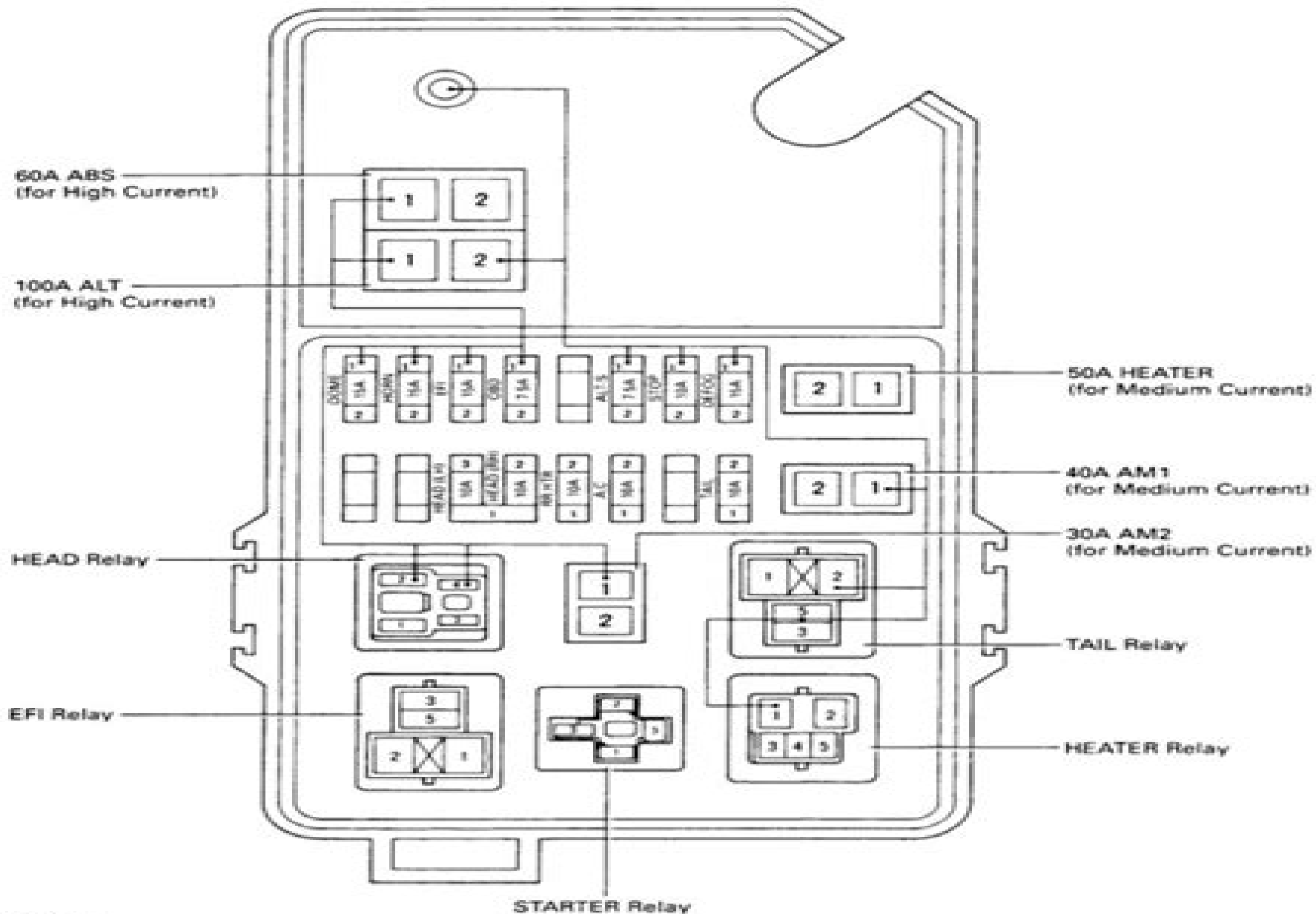
Engine Room R/B Components (USA)
