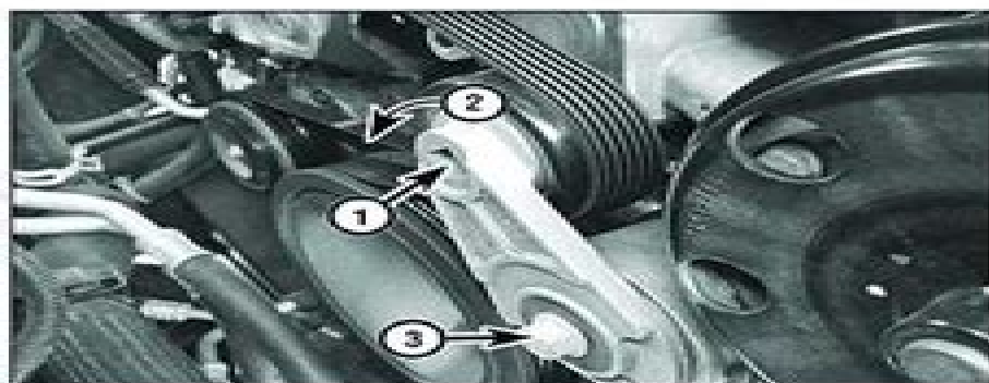
12.6b V8 engine accessory drivebelt tensioner details
