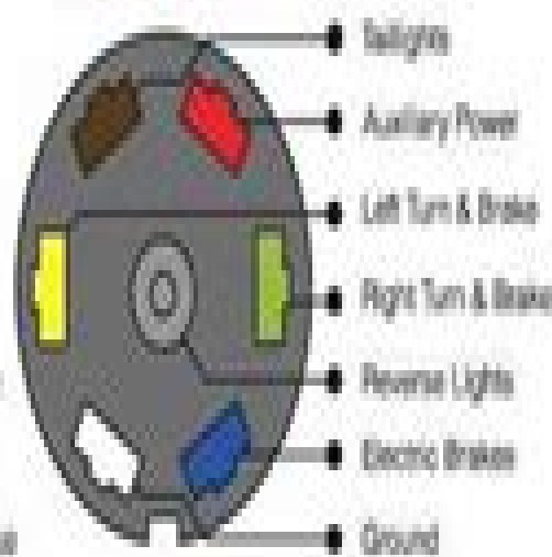
7 RV Blade
