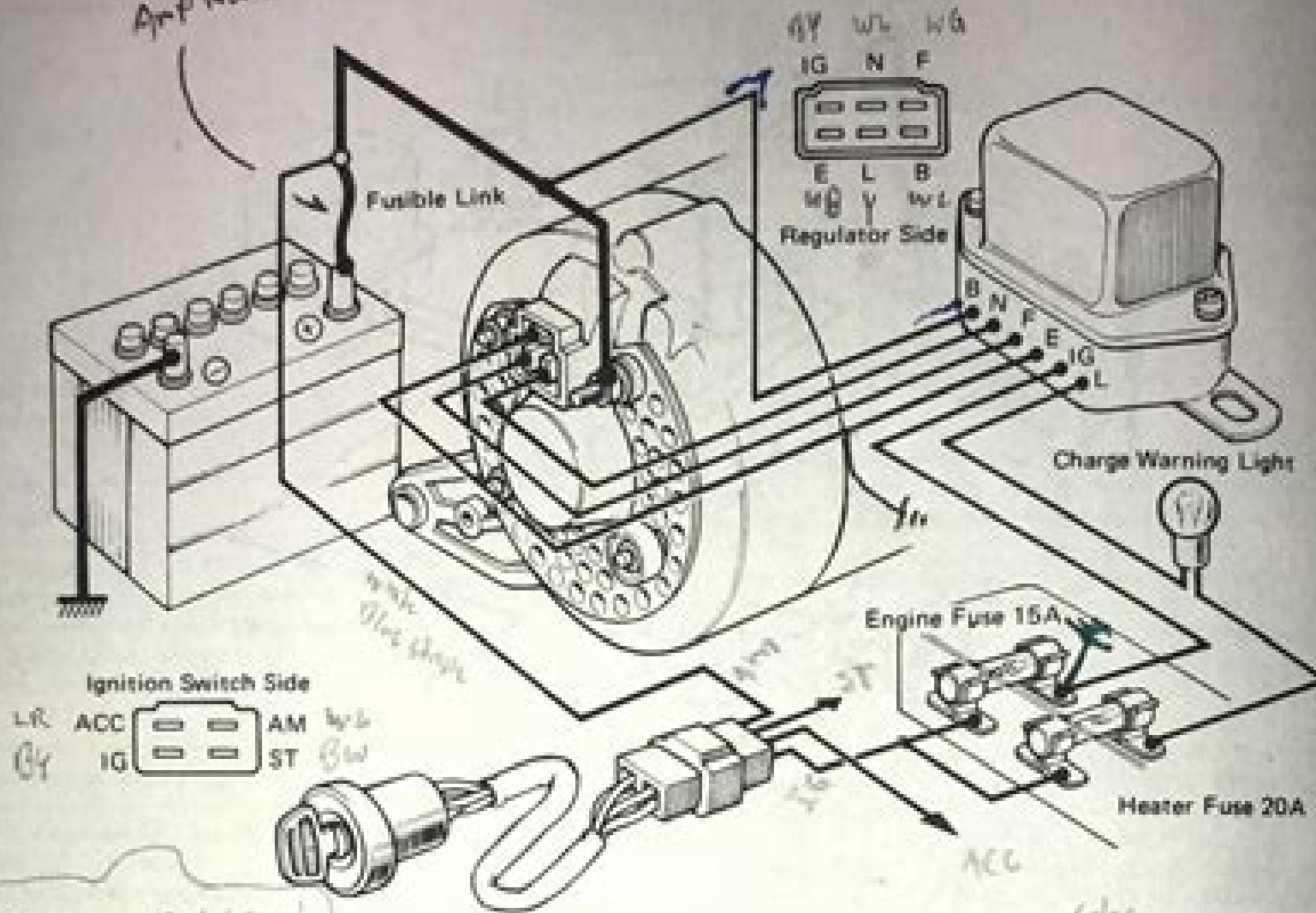
Fig. 11.2. Alternator connections - charge warning light types
