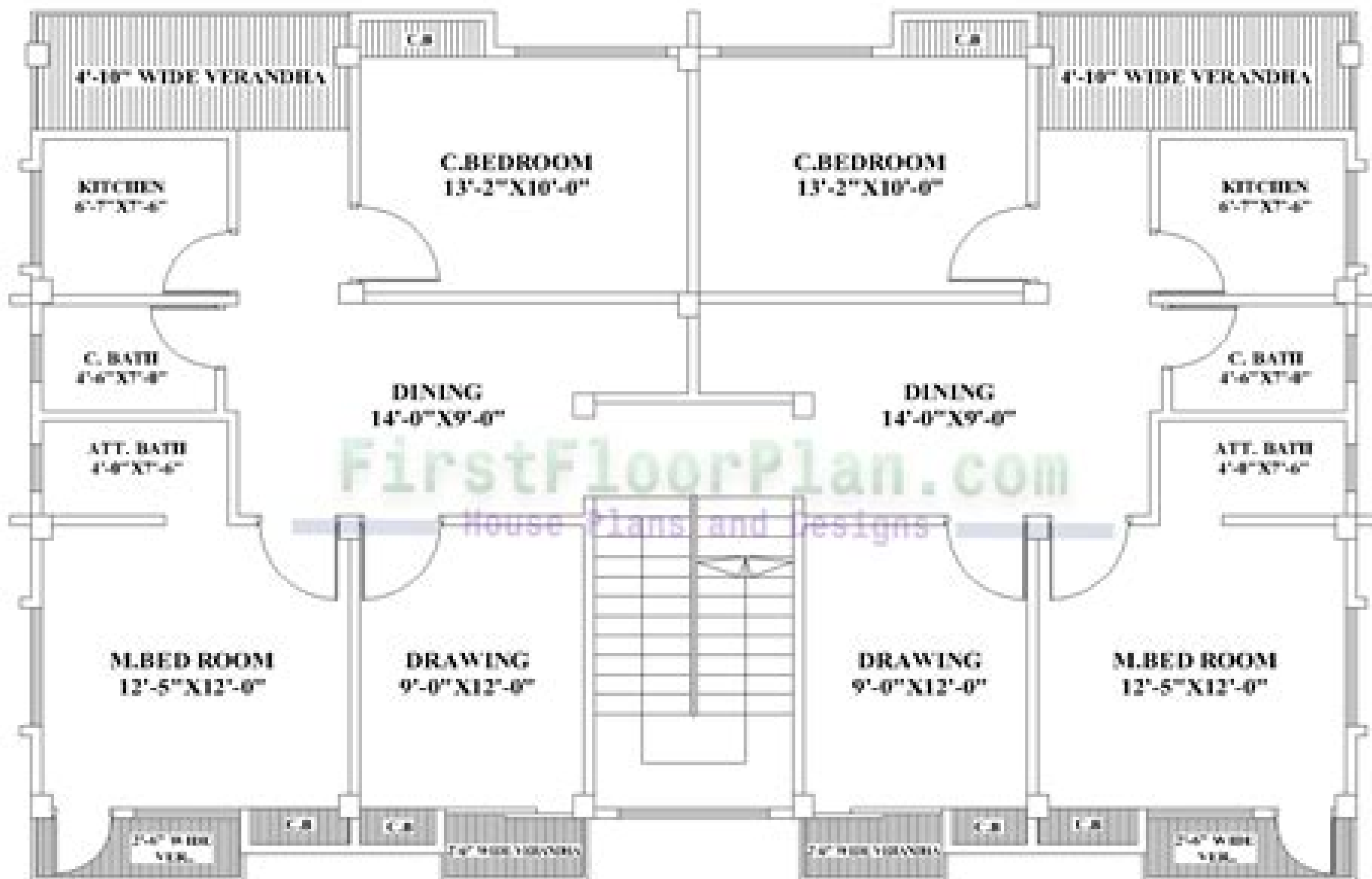
TYPICAL FLOOR PLAN FLOOR AREA: 2000 sq. ft.
