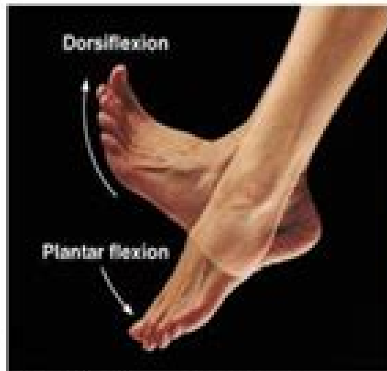
(e) Dorsiflexion and plantar flexion
