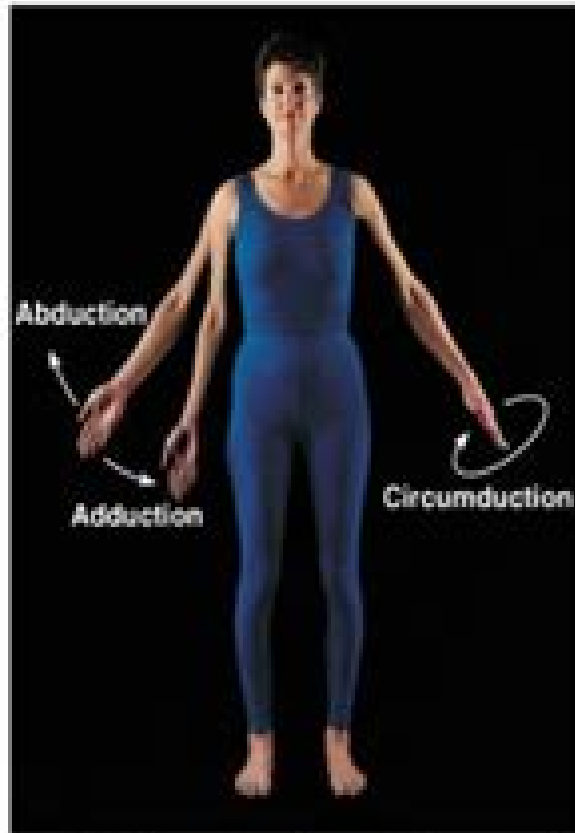
(d) Abduction, adduction, and circumduction
