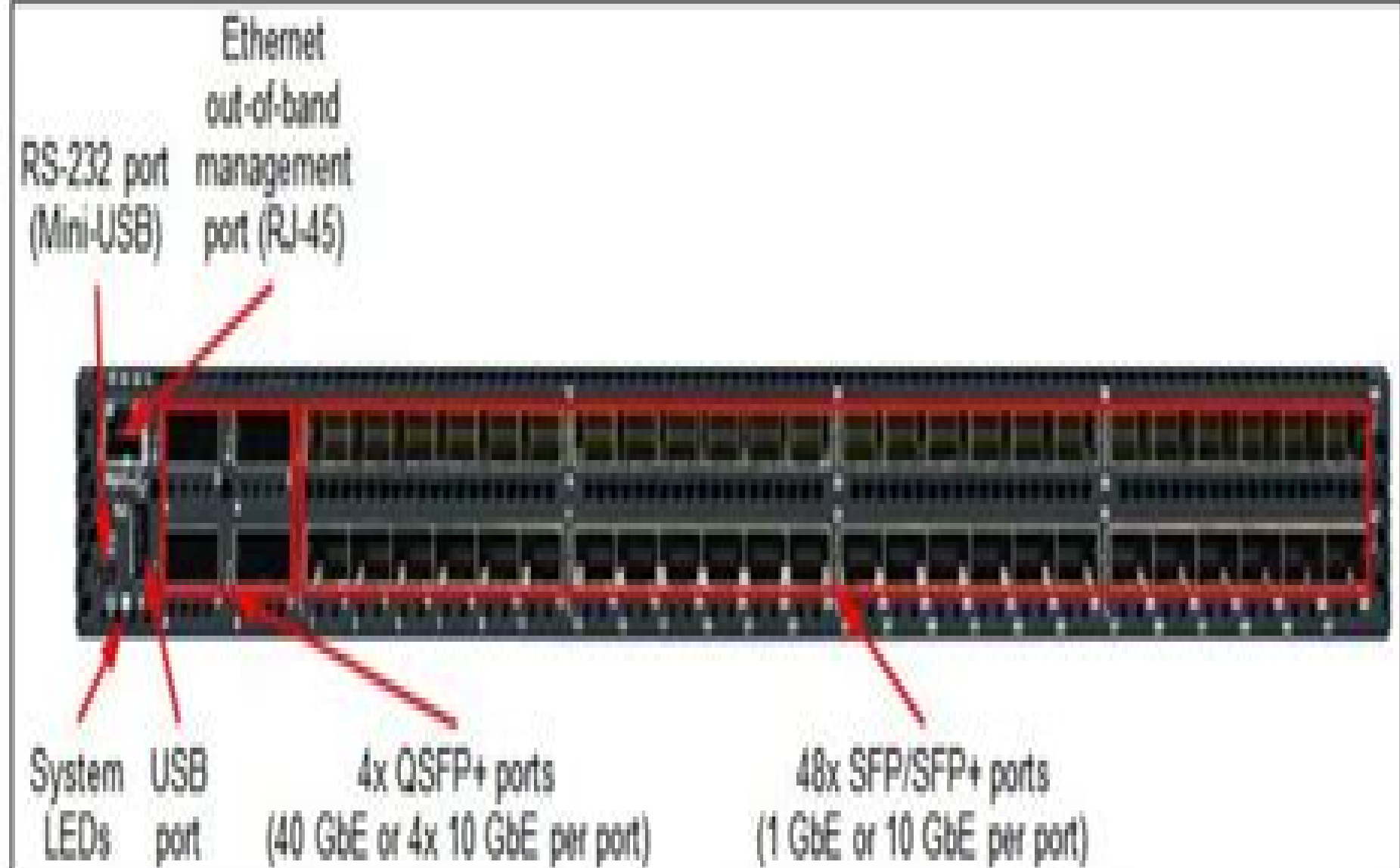
Figure 2. Front panel of the RackSwitch G8264
