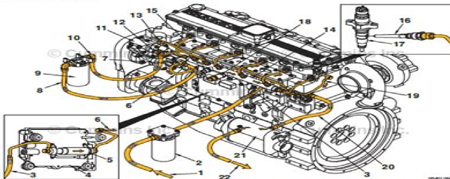
QSC8.3 Marine Applications (Sea Water Cooled), Cummins® Common Rail Fuel System Without ECM Fuel Cooling
