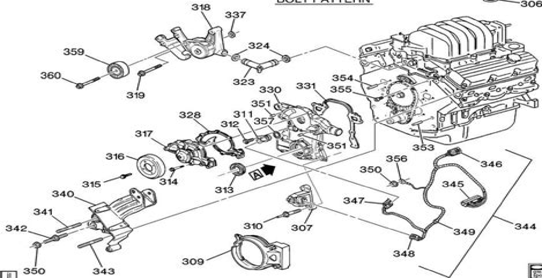
VIEW A FRONT COVER BOLT PATTERN
