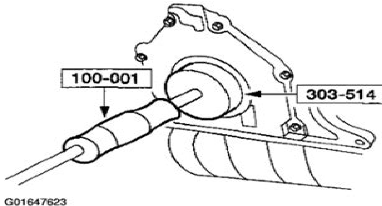
Fig. 726: Removing Crankshaft Rear Oil Slinger Courtesy of FORD MOTOR CO.
