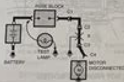
Figure 5 - Short Check
