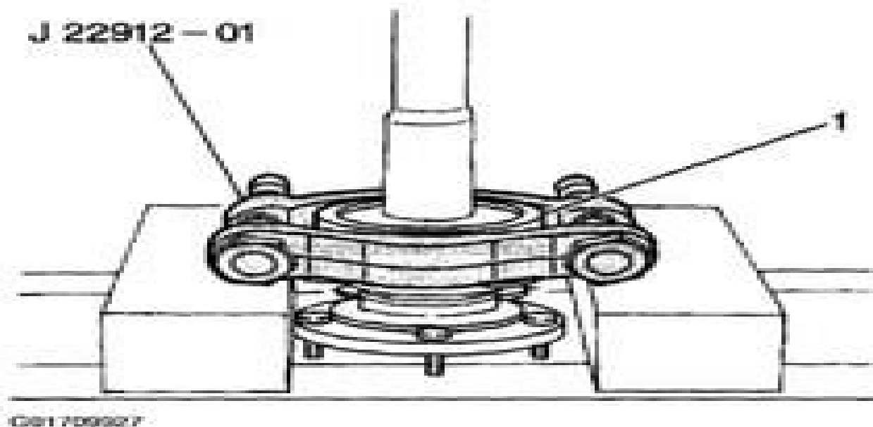
Fig. 17: Pressing Off Rear Axle Shaft Bearing From Rear Axle Shaft Courtesy of GENERAL MOTORS CORP.
